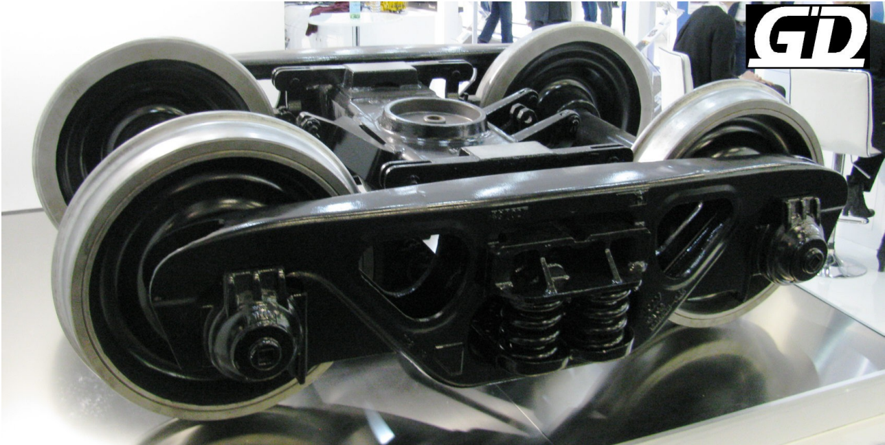
Güterwagen-Drehgestell Titagarh/AFR/SM "T Bogie-Family" (Schmalspur, T16/1000 mm - T 17/1067 mm) Freight Car Bogie Titagarh/AFR/SM "T Bogie-Family" (narrow gauge, T 16/1000 mm - T 17/1068 mm)
